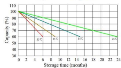
Temperature effects on capacity at 0.2C
